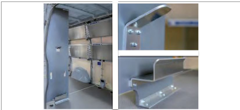
Figure 5: Hand truck mount without dolly (left), details (right)
